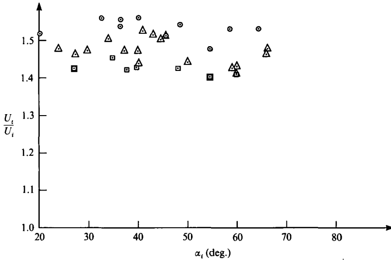
FIGURE 7. Comparison of the wave speed ratio U_t/U_i (see figure 2c) for a \text{CO}_2/\text{CH}_4 gas interface with \xi_i = 0.78 . \odot , Computed data for pure gases; \square , computed data for 10% contamination of the \text{CH}_4 by the \text{CO}_2 ; \triangle , experimental data (from Abd-El-Fattah & Henderson 1978b).
