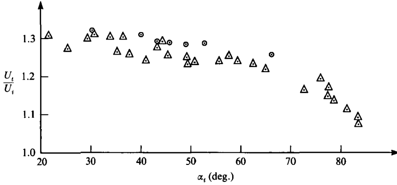
FIGURE 11. Comparison of the wave speed ratio U_i/U_i (see figure 2c) for a \text{CO}_2/\text{CH}_4 gas interface with \xi_i = 0.18 . \odot , Computed data for pure gases; \triangle , experimental data (from Abd-El-Fattah & Henderson 1978b).
