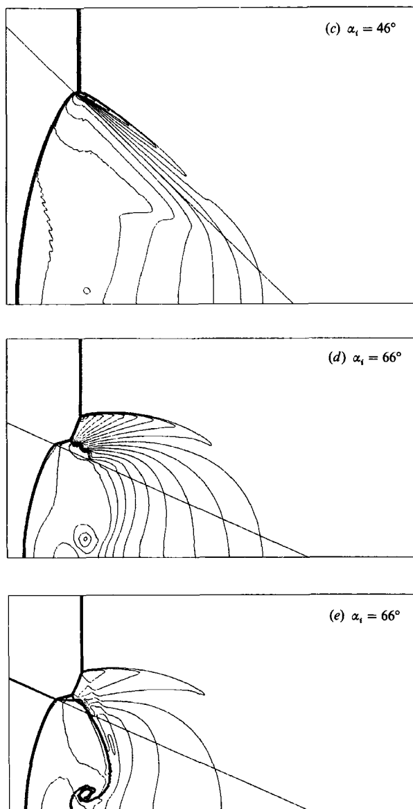
FIGURE 8. Contour plots of (a-d) \log P and (e) \log \rho from computations of a strong shock refraction sequence, \xi_1 = 0.18 , at a pure \text{CO}_2/\text{CH}_4 gas interface. (The straight line running diagonally from upper left to lower right represents the initial, undisturbed gas interface. It is not a pressure contour.)
