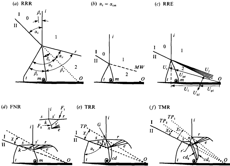
FIGURE 2. (a-c) Regular and (d-f) irregular shock refraction systems for a slow-fast \text{CO}_2/\text{CH}_4 gas interface, n < 1 . (a) Reflected shock, RRR, |Z_i| > |Z_r| , \alpha_i > \alpha_r ; (b) reflected Mach line degeneracy, |Z_i| = |Z_r| , \alpha_i > \alpha_r = \alpha_{im} ; (c) reflected expansion, RRE, |Z_i| < |Z_r| , \alpha_i > \alpha_r ; (d) free precursor von Neumann refraction, FNR; (e) twin regular reflection-refraction, TRR; (f) twin Mach reflection-refraction, TMR. i , Incident shock; t , transmitted shock; r, r' , reflected shocks; e , reflected expansion wave; k , modified incident shock; n , Mach shock; s , side shock; s' , modified side shock; m , gas interface; I, Region of undisturbed \text{CO}_2 ; II, region of undisturbed \text{CH}_4 ; MW , Mach line; cd_{(1,2)} , contact discontinuity; TP_{(1,2)} , trajectory path of shock wave confluences; \chi_{(1,2)} , trajectory path angles of shock wave confluences; F_{1,2} , shock triple points; G , quadruple point; O origin where i first encountered gas interface.
