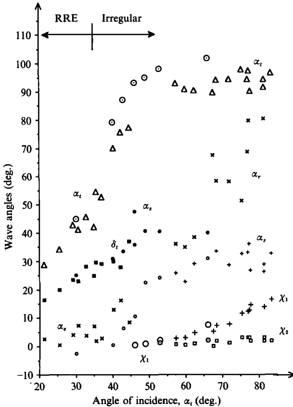
FIGURE 12. Experimental and computational wave angle data for a \text{CO}_2/\text{CH}_4 refraction with \xi_i = 0.18 . Circular symbols represent data from computations with pure gases. All other symbols represent experimental data. \odot , \triangle , Transmitted shock angle \alpha_t ; \circ , \times , reflected wave angle \alpha_r or \alpha_r ; \bullet , + , side shock angle \alpha_s ; \odot , \square , interface deflection angle \delta_i ; \odot , + , trajectory path angle \chi_1 ; \odot , \square , trajectory path angle \chi_2 . (Experimental data from Abd-El-Fattah & Henderson 1978b.)
