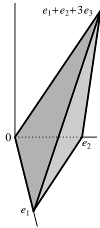
Figure 3. The simplex P = \text{Conv}(0, e_1, e_2, e_1 + e_2 + 3e_3) \subseteq \mathbb{R}^3
