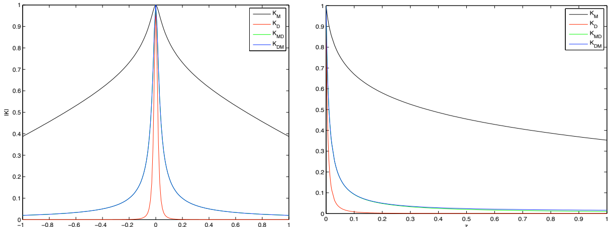
FIGURE 2. (Left) 3d transverse profiles with FWHM = 1.37(K_M), 0.03(K_D), 0.07(K_{MD}, K_{DM}) ; (Right) 3d longitudinal profiles with FWHM = 0.3565(K_M), 0.00421(K_D), 0.00947(K_{DM}, K_{MD}) . Note that the transverse profiles of the K_{MD} and K_{DM} coincide.
