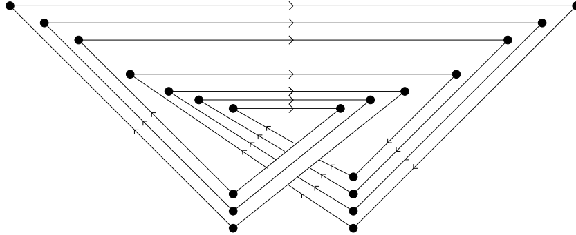
Figure 2: Knot diagram of polygon P_3 .
