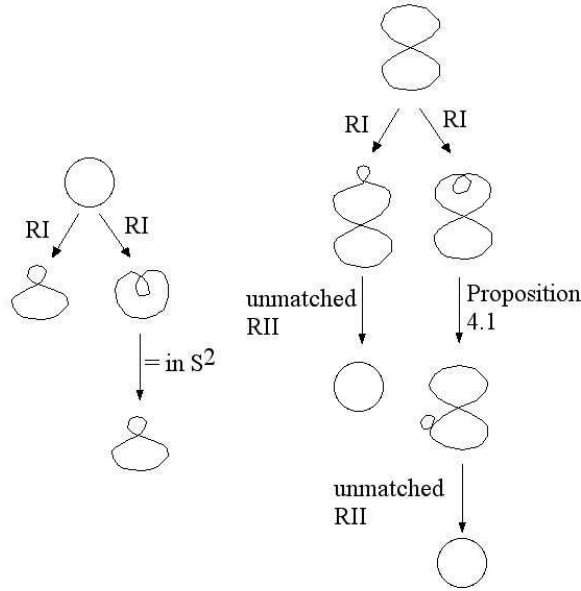
Figure 11: A is unchanged by the introduction of a kink.
