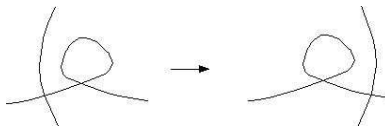
Figure 8: A kink slides across an arc.
