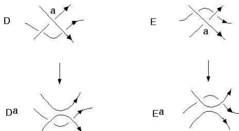
Figure 4: Links arising from smoothings of RIII moves involving the top and middle strand
