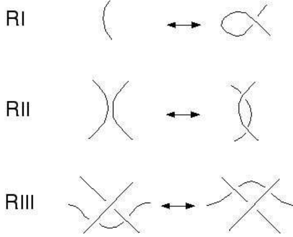
Figure 2: Reidemeister moves
