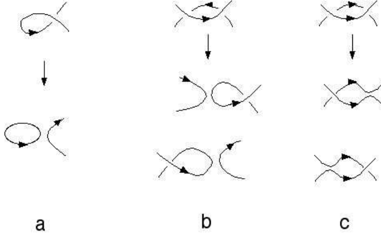
Figure 3: Links arising from smoothing after RI and RII moves
