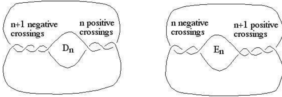
Figure 6: An unknot D_n and its mirror image E_n
