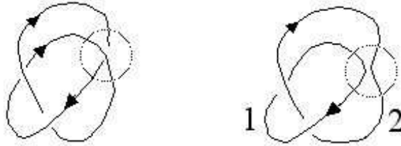
Figure 1: A smoothing results in a 2-component link
