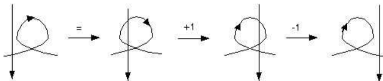
Figure 9: The value of A is invariant under these moves.
