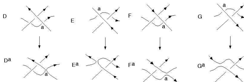
Figure 5: The links arising from smoothings of RIII moves involving the top and bottom strand
