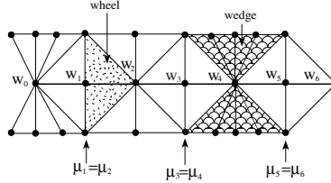
Figure 4: A 2-dimensional section of R_K .
