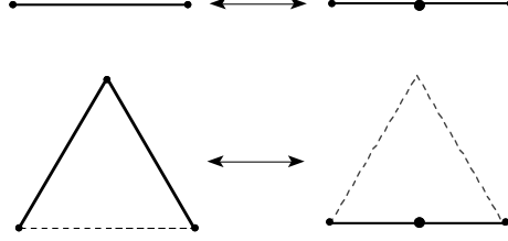
Figure 2: Two types of elementary moves.
