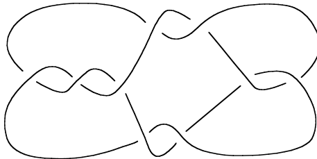
Figure 1: Goeritz's unknot.
