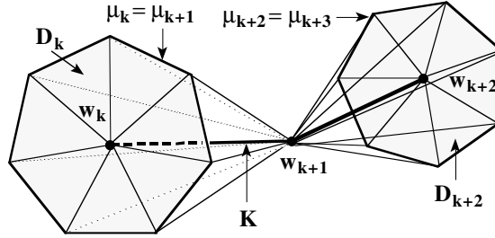
Figure 5: Adjacent meridians. The index k is odd.
