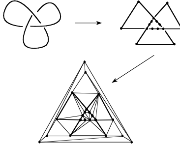
Figure 14: Triangulating a knot projection.
