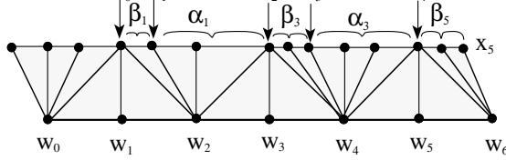
Figure 6: The annulus S_0 .
