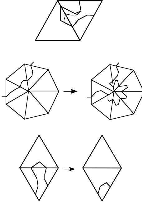
Figure 11: Basic move of types 1, 2 and 3.
