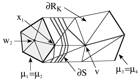
Figure 8: Adding twists replaces S_0 by S .
