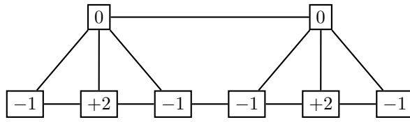
Fig. 3.6. Laplacian \mathbf{L} , \lambda_5 = 4 (multiplicity r = 2 ).
