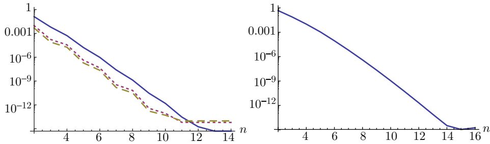
FIGURE 3. The maximum error in approximating the Hilbert transform of e^x by 2i\mathcal{M}_{\mathbb{I},n}f over 200 evenly spaced points on circles of radii 2 (left graph, plain), 25 (left graph, dotted) and 50 (left graph, dashed) and by i(\mathcal{M}_{\mathbb{I},n}^+f + \mathcal{M}_{\mathbb{I},n}^-f) at 200 evenly spaced points on the unit interval (right graph)
