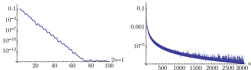
FIGURE 4. The maximum error over the points R(\ddagger_{10}) of (6.1) (left graph) and (4.2) (right graph) for approximating the Hilbert transform of \frac{\arctan y}{y} . Note that the value on the bottom axis corresponds to the total number of function evaluations
