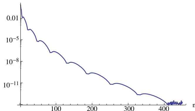
FIGURE 2. The maximum error in approximating the Hilbert transform of \frac{1-\text{sech } y}{y} by (4.2) at the points R(z_n)
