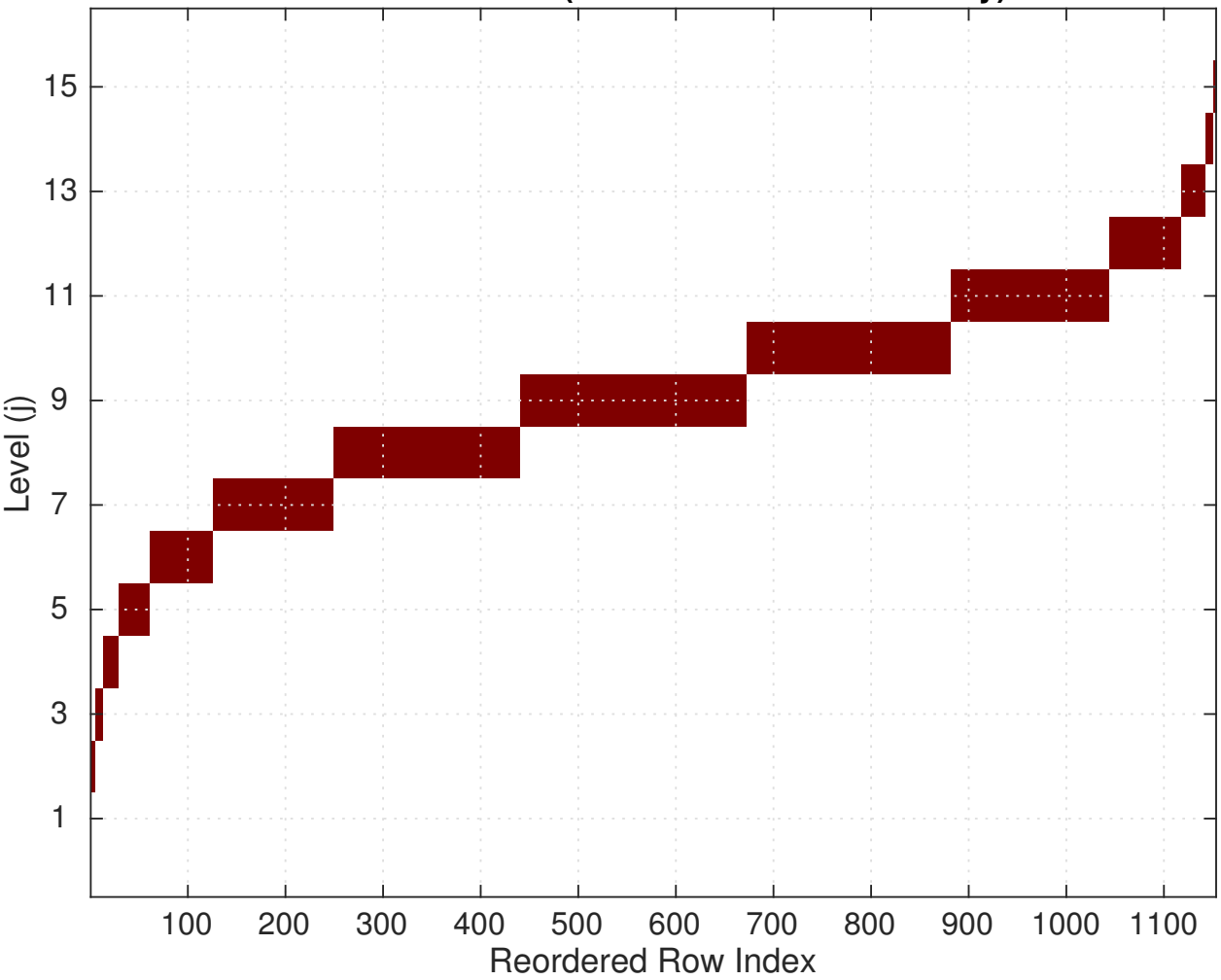
Row Haar Basis (Fine-To-Course Dictionary)
