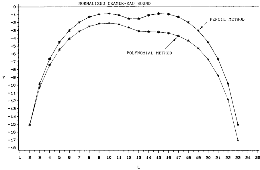
Fig. 1. This plot shows 10 \log_{10} (\text{CRB}/\text{Var}(\delta f_i)) versus L where \text{Var}(\delta f_i) ("**") was computed from perturbation analysis. The signal parameters are M = 2 , N = 25 , \alpha_1 = -0.01 , \alpha_2 = -0.02 , f_1 - f_2 = -0.02 , and any \phi_1 and \phi_2 .
