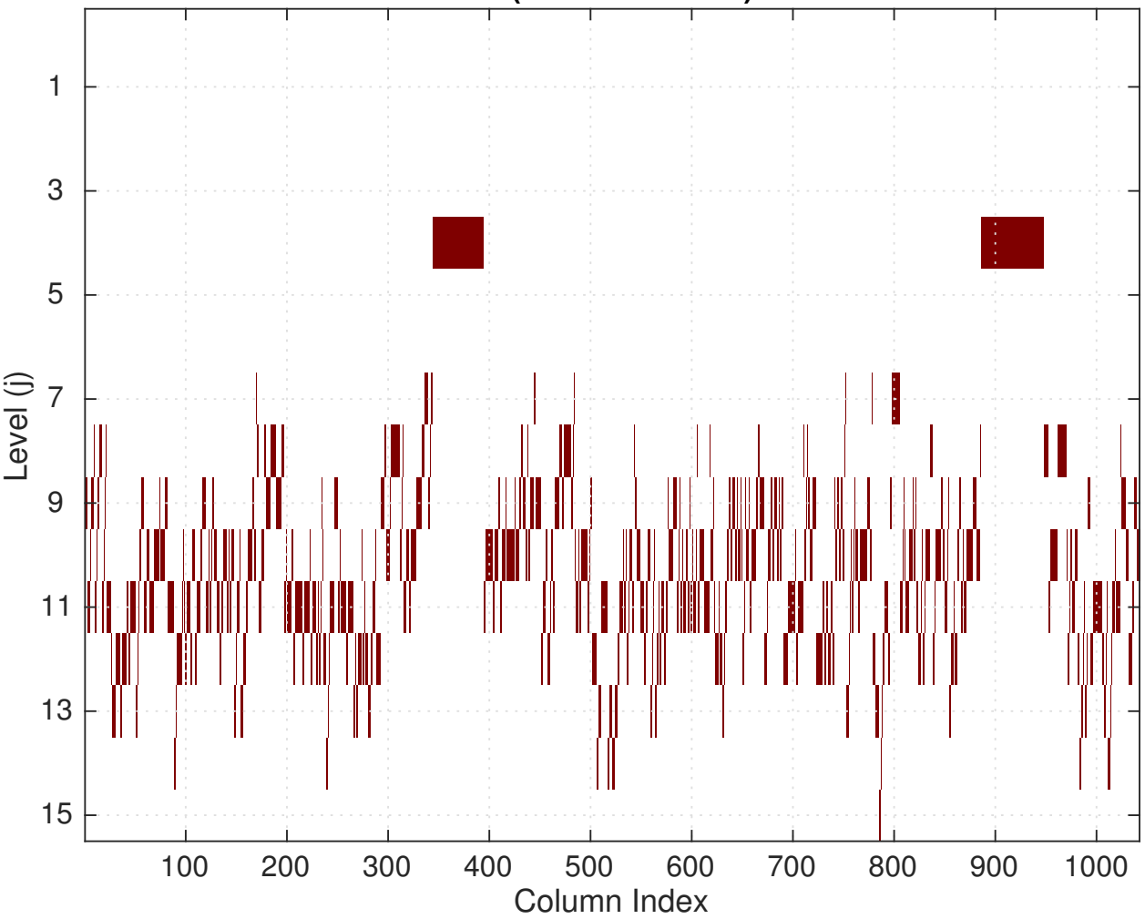
Column Best Basis (Coarse-to-Fine) Partition Pattern
