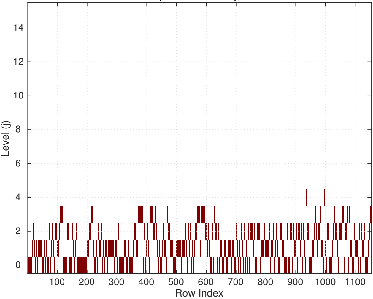
Row Best Basis (Fine-to-Coarse) Partition Pattern
